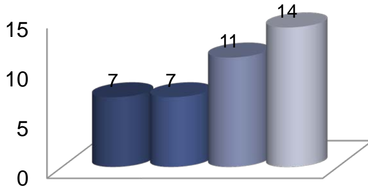
Nb Cyclo
